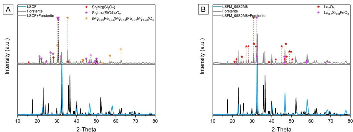
Figure 5: XRD for (A) LSCF–forsterite and (B) LSMF 95S2M8–forsterite (in grey; mixed pellet) after T < 1300^{\circ}\text{C} 5h. The spectra are shown for raw forsterite (black line) and for the raw cathode material (blue line).
